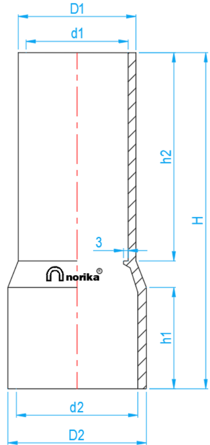
CROSS SECTION VIEW
